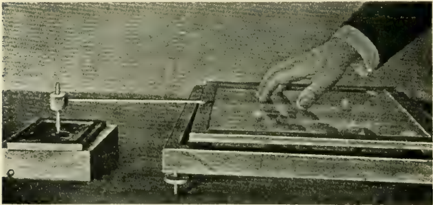
FIG. 1. — THE AUTOMATOGRAPH. When in use a screen (not shown in the illustration) cuts off the view of the apparatus from the subject. The recording device, which may also be used separately, is shown in outline in half its full size. R is a glass rod which moves freely up and down in the glass tube T, which is set into the cork C. A rubber band B is provided to prevent the rod from falling through the tube, when not resting upon the recording-plate.
